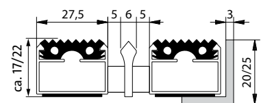
Portagard AK
