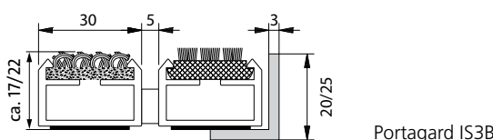
Portagard IS3B
