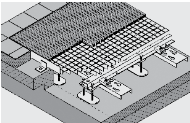
Substructure
