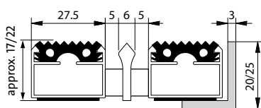
Portagard AK
