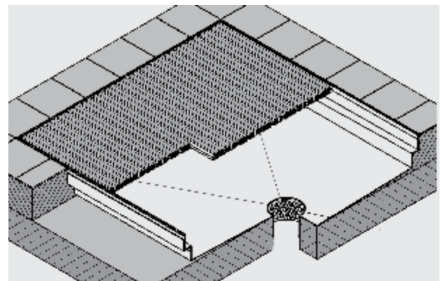
PortaDrain dirt collection well
